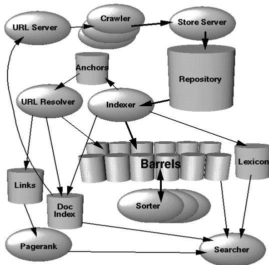
Figure 4: Google’s Search Engine Architecture
